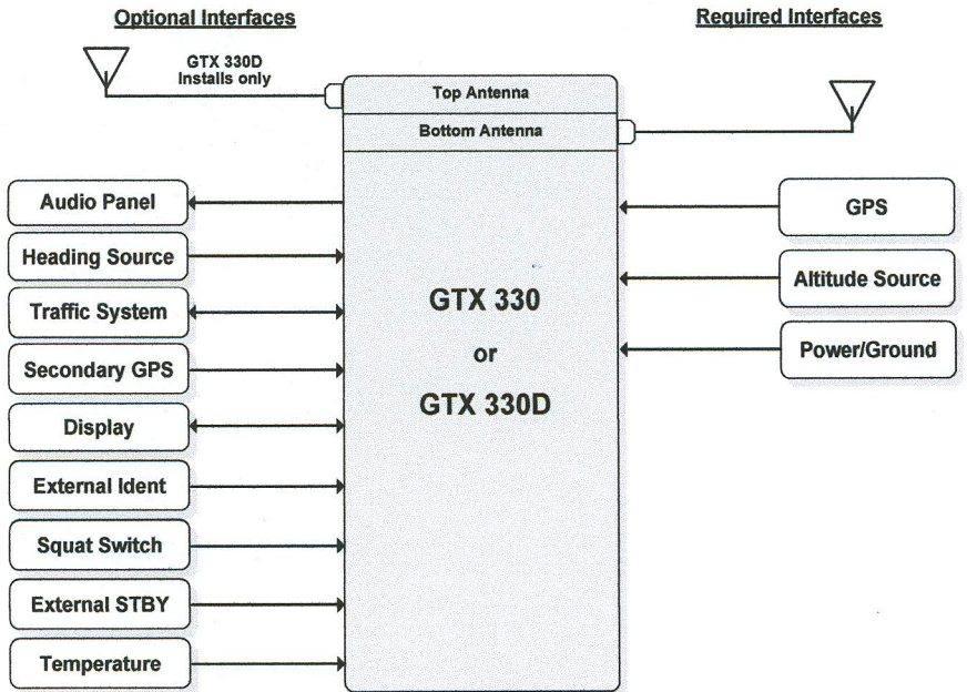
Figure 1 – GTX 330 or GTX 33D Interface Summary
